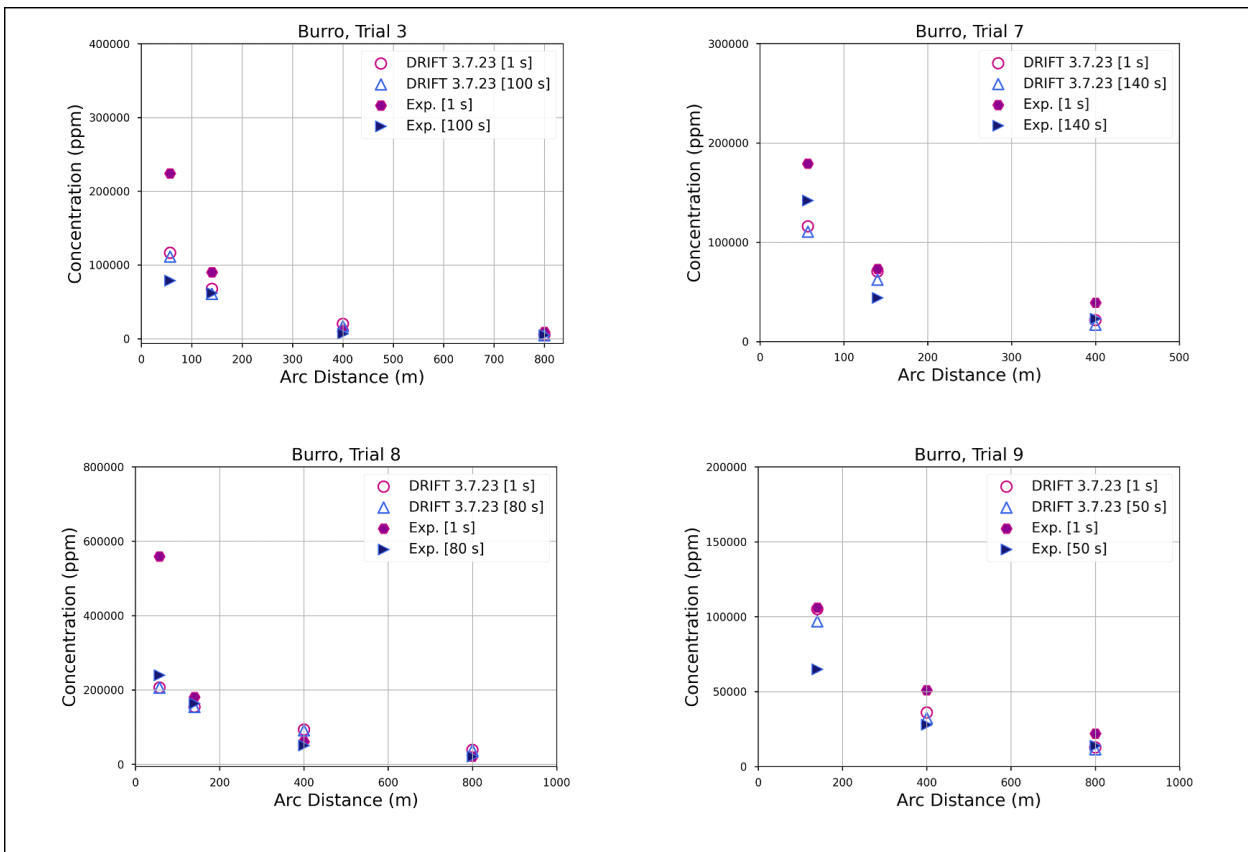
Figure 8 presents a comparison of the DRIFT 3.7.23 predictions with the Burro experimental data. There are considerable differences between the experimental concentrations obtained using the short and long averaging times. This difference between averaging durations is not evident for the DRIFT runs. For trials 3 and 8, DRIFT does not capture the peak instantaneous concentration values observed in the experiments.
