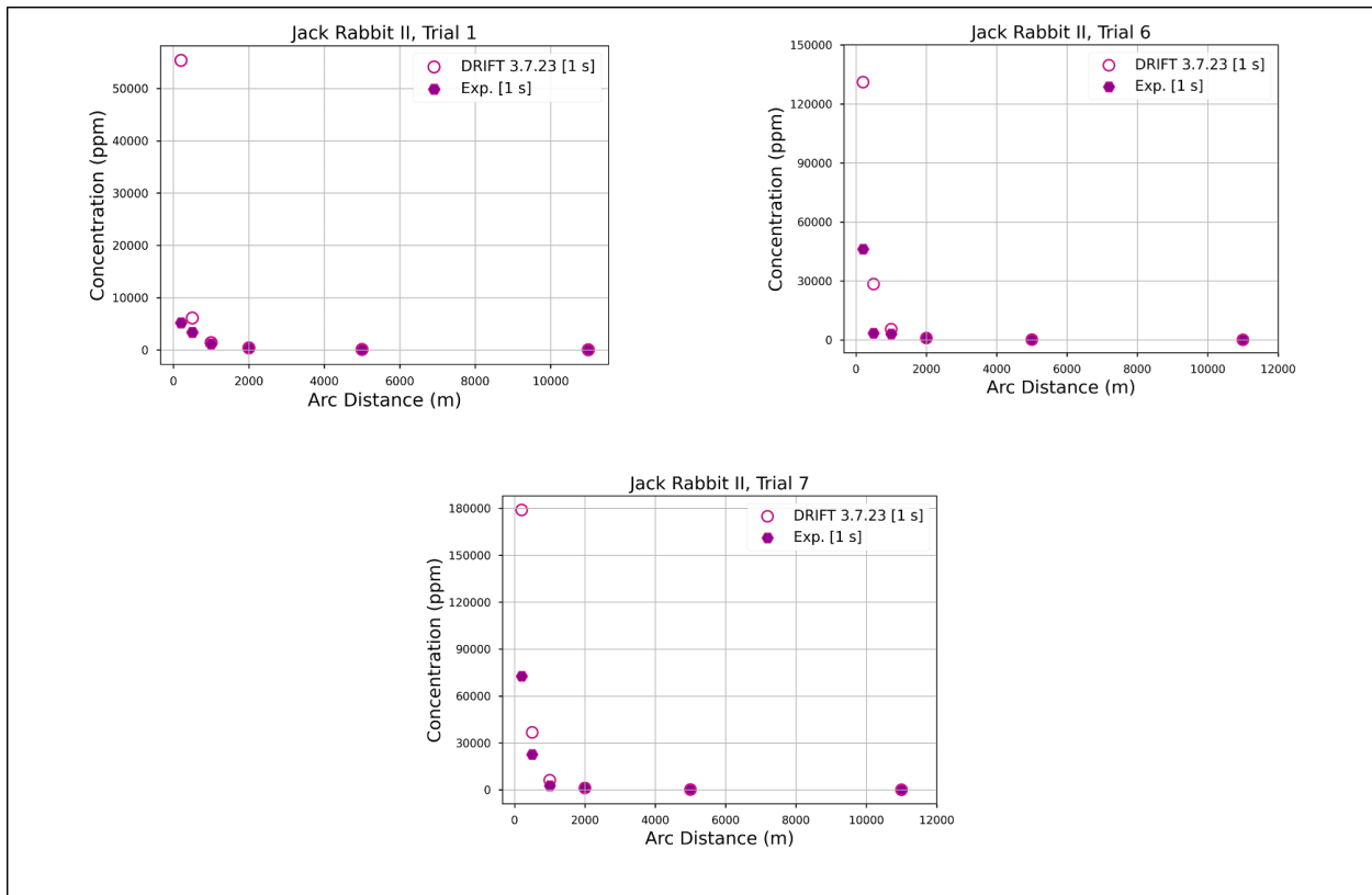
Figure 13 presents a comparison of the DRIFT 3.7.23 predictions with the Jack Rabbit II experimental data for trials 1, 6 and 7. DRIFT substantially overpredicts (by roughly a factor of 10) the concentration in trial 1 at the first sensor located at 200 m. However, as discussed in Gant et al. (2022), there were only 3 sensors on the arc at 200 m, and the plume centreline could have missed these sensors.
