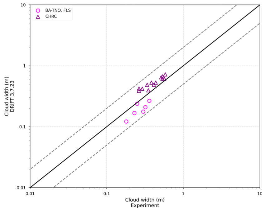
Figure 28 Long-time averaged cloud width data scatter for all wind-tunnel trials. Solid line indicates where predicted is equal to measured. Dashed lines indicate a factor of two under- and overprediction.
