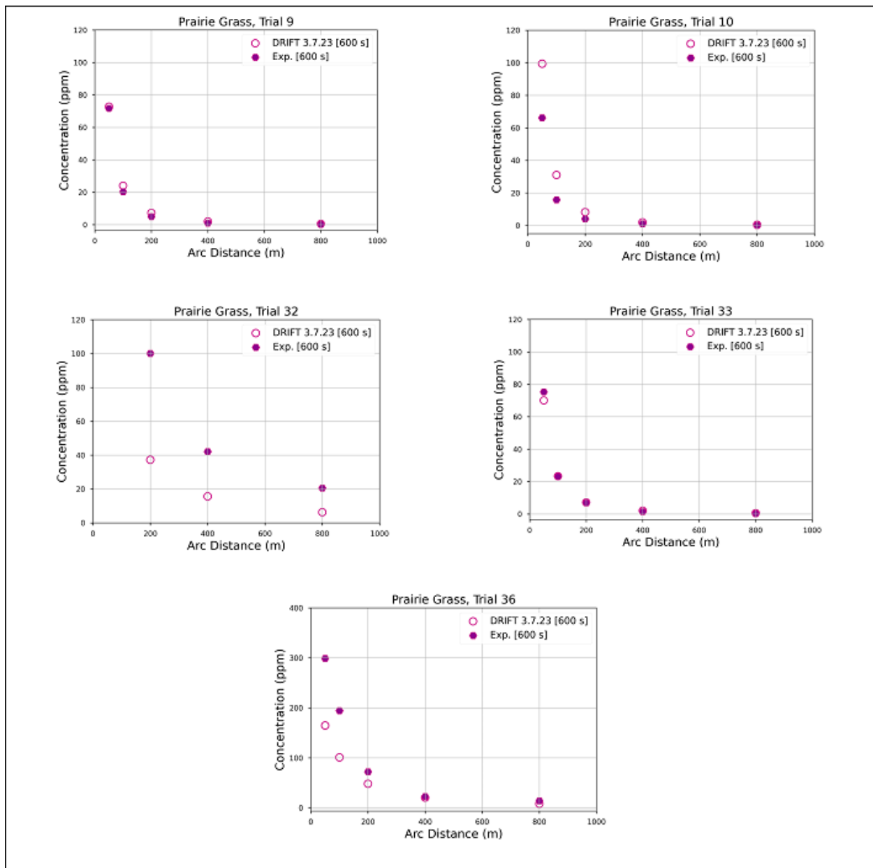
Figure 17 Observed and predicted maximum arcwise concentration data for Prairie Grass. Square brackets indicate averaging time.
