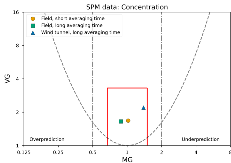
Figure 29 Geometric variance (VG) versus geometric mean bias (MG) based on concentration data.
