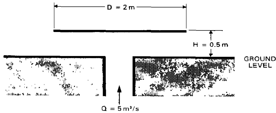
Figure 11 Thorney Island vertical duct source. Image from McQuaid (1987).
