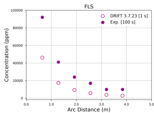
Figure 4 Observed and predicted maximum arcwise concentration data for BA-TNO FLS. Square brackets indicate averaging time.
