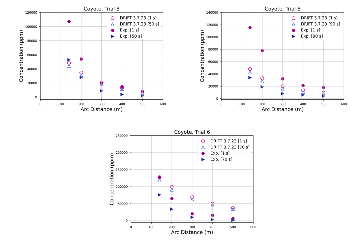
Figure 9 Observed and predicted maximum arcwise concentration data for Coyote. Square brackets indicate averaging time.
