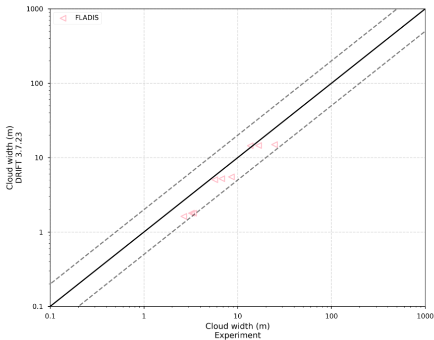
Figure 26 Short-time averaged cloud width data scatter for the FLADIS field trials. Solid line indicates where predicted is equal to measured. Dashed lines indicate a factor of two under- and overprediction.
