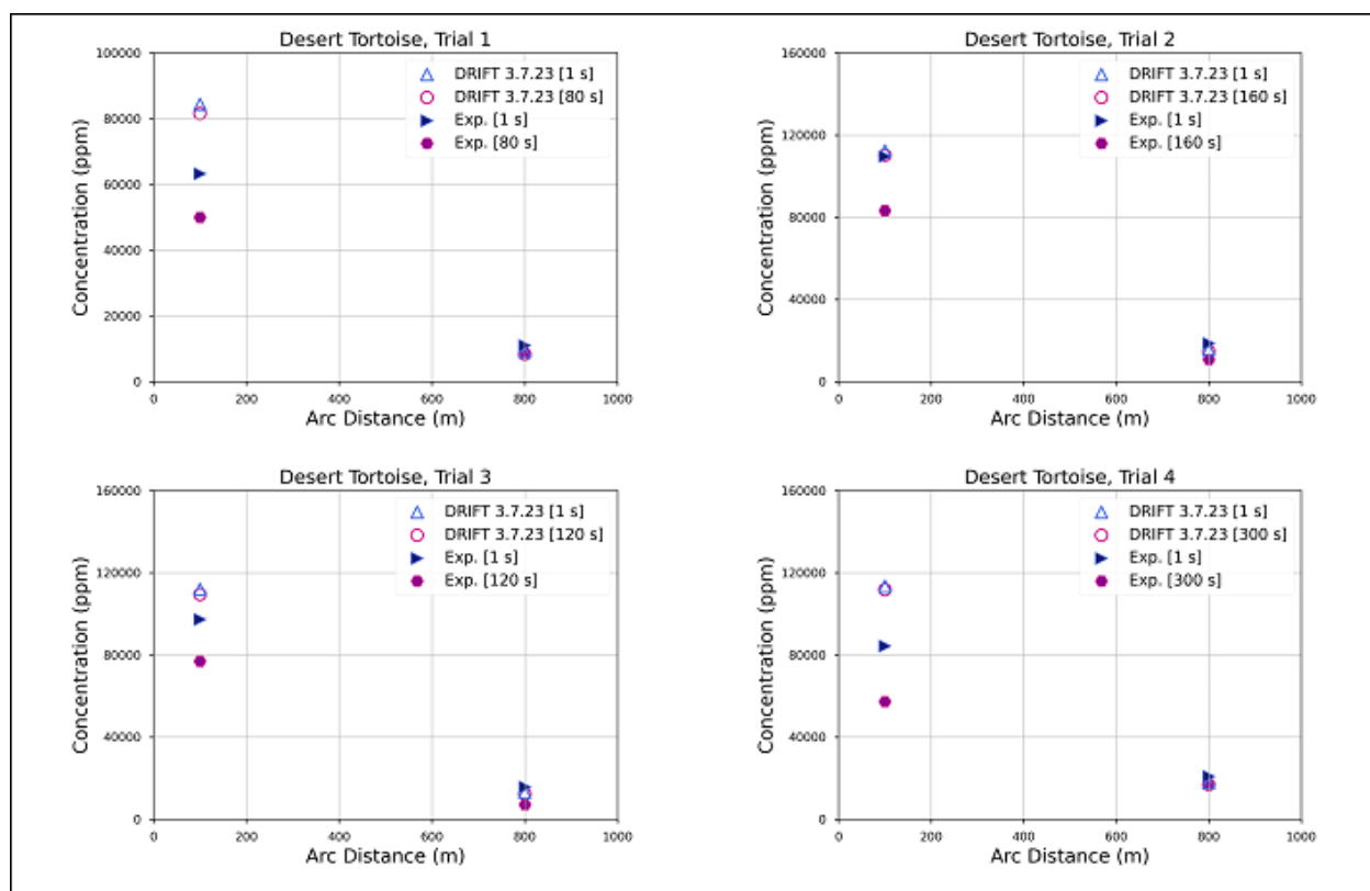
Figure 18 presents a comparison of the DRIFT predictions with the Desert Tortoise data.
