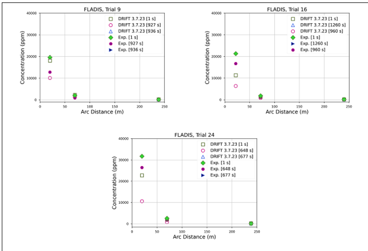
Figure 19 Observed and predicted maximum arcwise concentration data for FLADIS. Square brackets indicate averaging time.
