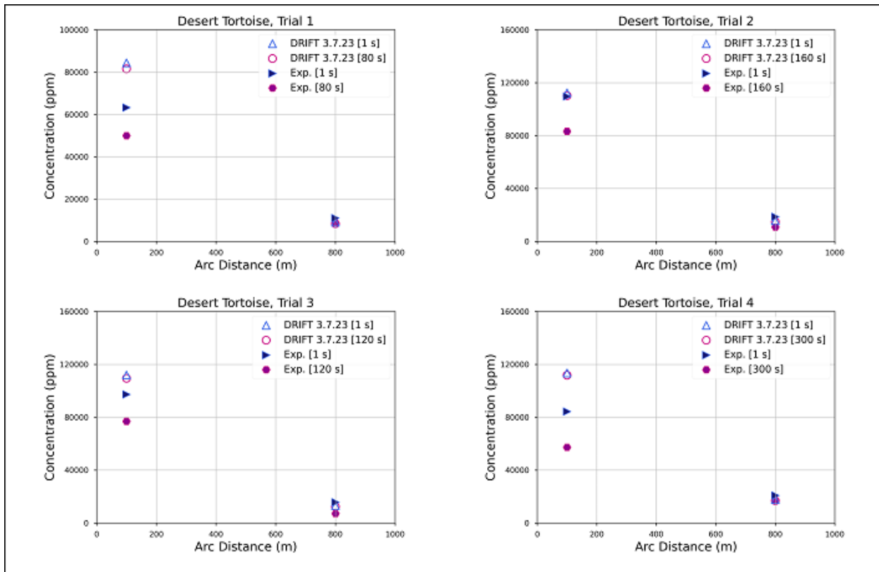
Figure 18 Observed and predicted maximum arcwise concentration data for Desert Tortoise. Square brackets indicate averaging time.
