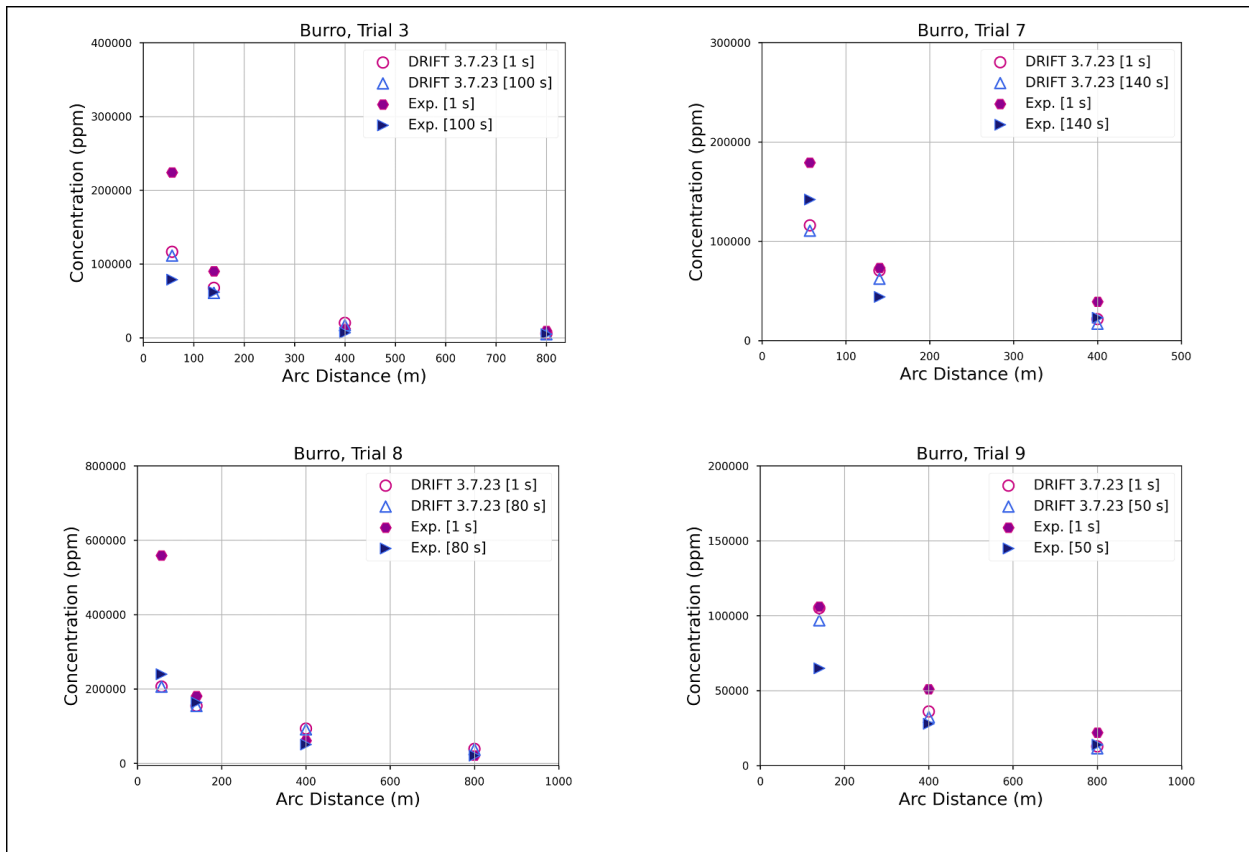
Figure 8 Observed and predicted maximum arcwise concentration data for Burro. Square brackets indicate averaging time.
