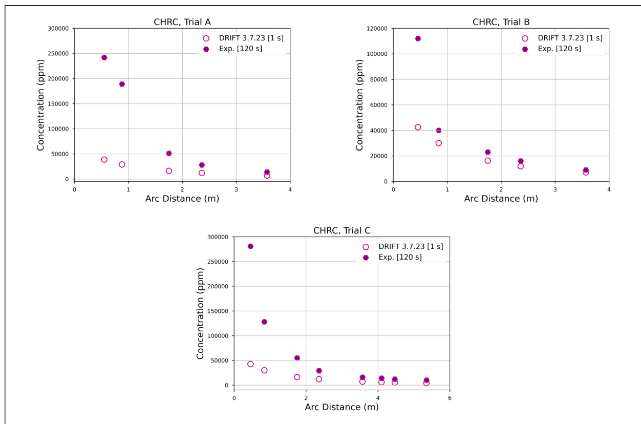
Figure 5 presents a comparison of the DRIFT predictions with the CHRC experimental
