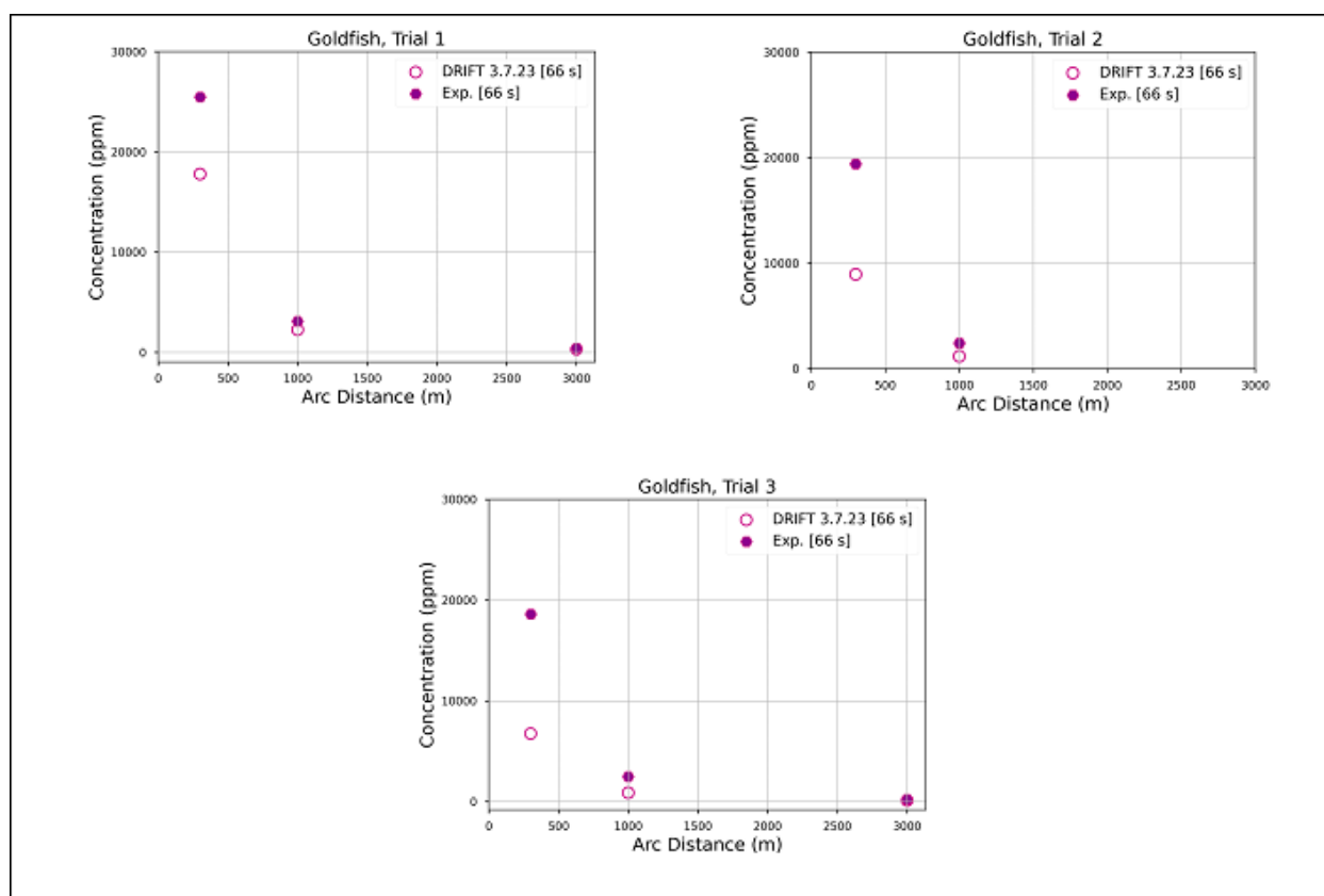
Figure 20 Observed and predicted maximum arcwise concentration data for Goldfish. Square brackets indicate averaging time.
