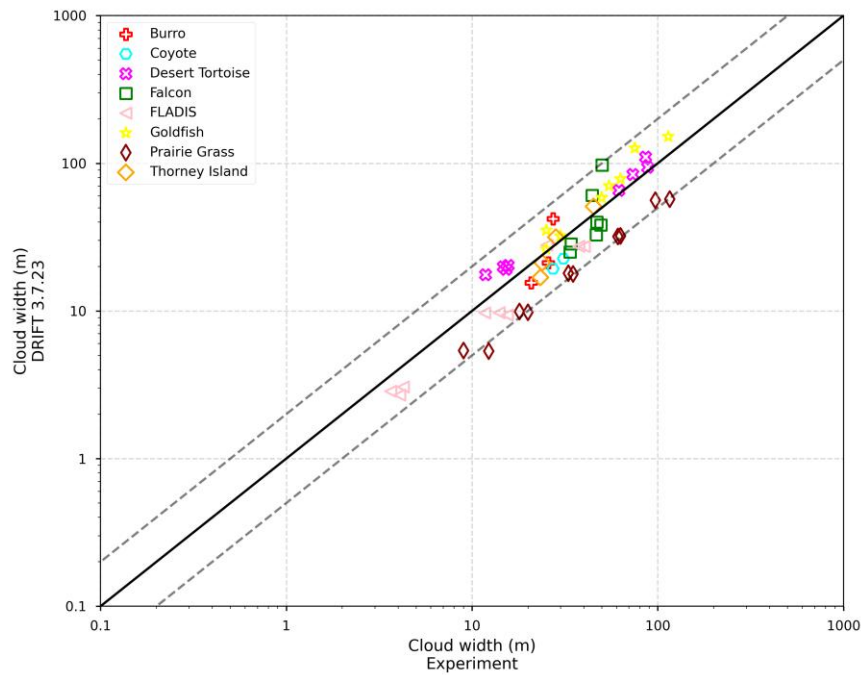
Figure 27 Long-time averaged cloud width data scatter for all field trials. Solid line indicates where predicted is equal to measured. Dashed lines indicate a factor of two under- and overprediction.
