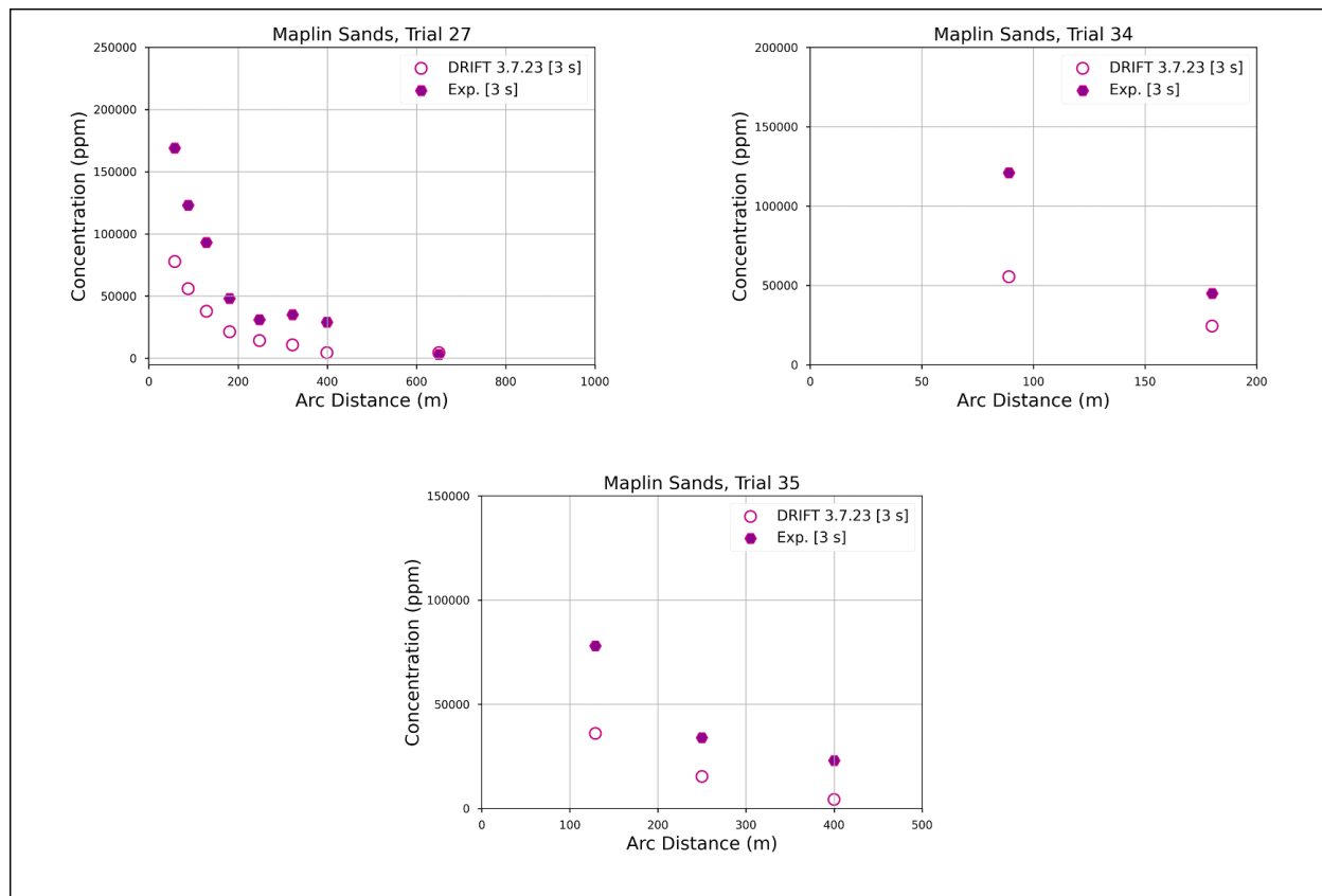
Figure 6 presents a comparison of the DRIFT 3.7.23 predictions with the Maplin Sands experimental data. For all the Maplin Sands trials, DRIFT underpredicts the measured concentrations. Hanna et al. (1993a,b) tested 14 hazard response models against eight gas dispersion experiments, including Maplin Sands, and several models within that study also reported significant underpredictions. Uncertainties in the Maplin Sands data are summarised in Stewart et al. (2016) and Batt (2021). These include poor sensor coverage and high winds causing narrow plumes to miss sensors. In addition, there was no splash plate to direct the source radially across the pond, and it is likely that the resulting plunging jet source led to greater dispersion than would have occurred from an area source. Stewart et al. (2016) recommend running sensitivity analysis on the source conditions due to the uncertainty in the vaporisation rate.
