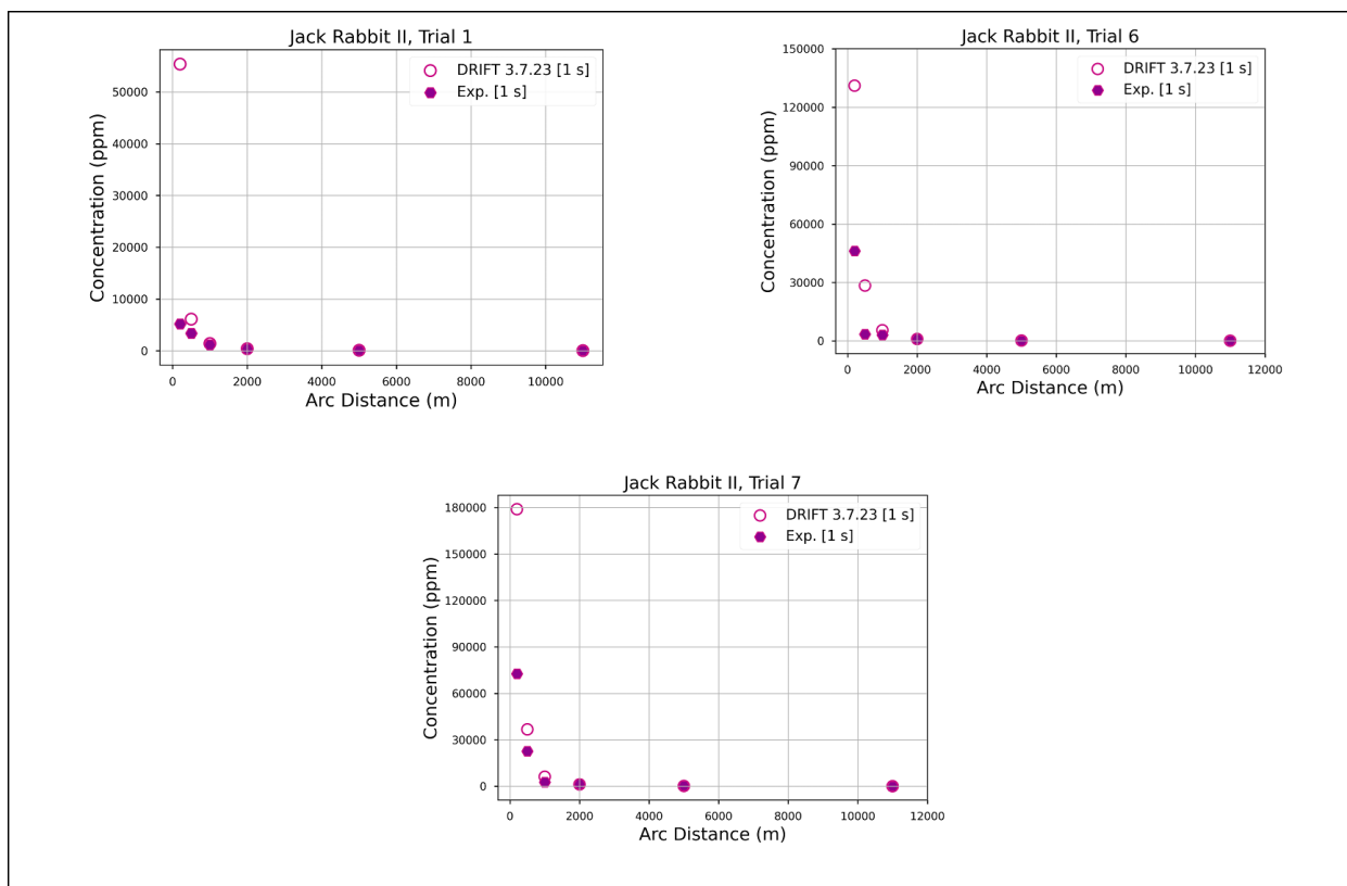
Figure 13 Observed and predicted maximum arcwise concentration data for Jack Rabbit II. Square brackets indicate averaging time.
