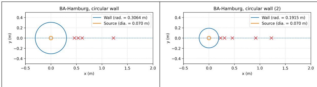
Figure 3 presents scale drawings of both trials. Poor agreement between the measured and predicted concentrations for the first circular wall trial could be due to the size difference between the 70 mm source and the circular wall.
