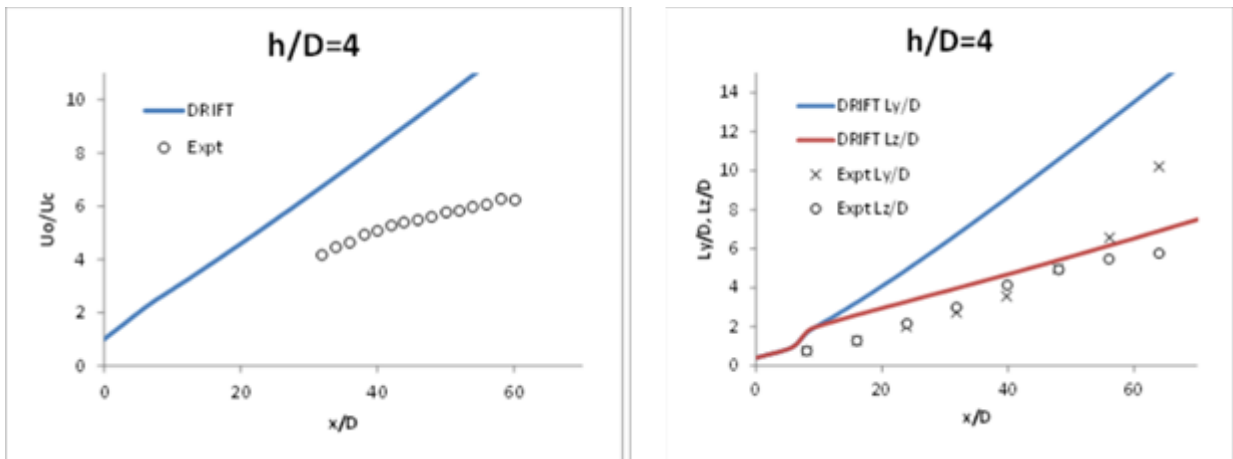
Figure 34 DRIFT 3.6.14 predictions of velocity and plume dimensions for h/D = 4 compared with Davis and Winarto (1980) data. Reproduced from Figure 2-5 of Tickle (2025c).
