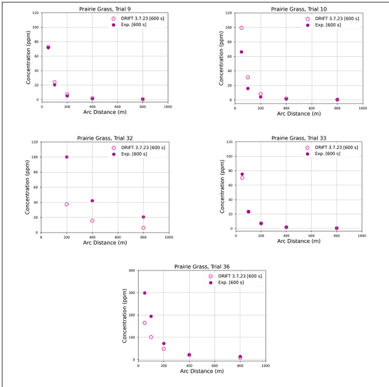
Figure 17 presents concentration data for Prairie Grass trials 9, 10, 32, 33 and 36. DRIFT 3.7.23 predictions are especially close to the experimental data for trials 9 and 33, where the wind speed is high and the stability ranges from neutral to slightly unstable. Trials 32 and 36 show model underprediction, roughly by a factor of 2. These trials are both Pasquill stability class F (stable), and relatively low wind speed. Trial 10 (Pasquill class B, unstable) displays the opposite behaviour, as DRIFT reports concentrations higher than those observed experimentally. These findings are consistent with previous investigations of Prairie Grass using DRIFT, see for example Tickle (2012).
