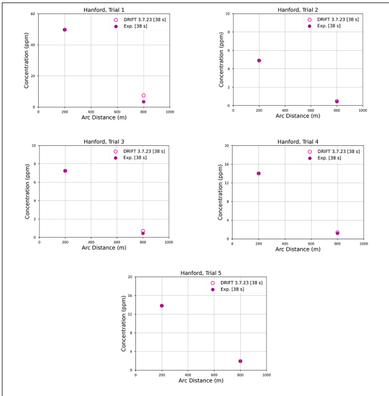
Figure 15 Observed and predicted maximum arcwise concentration data for continuous Hanford trials. Square brackets indicate averaging time.
