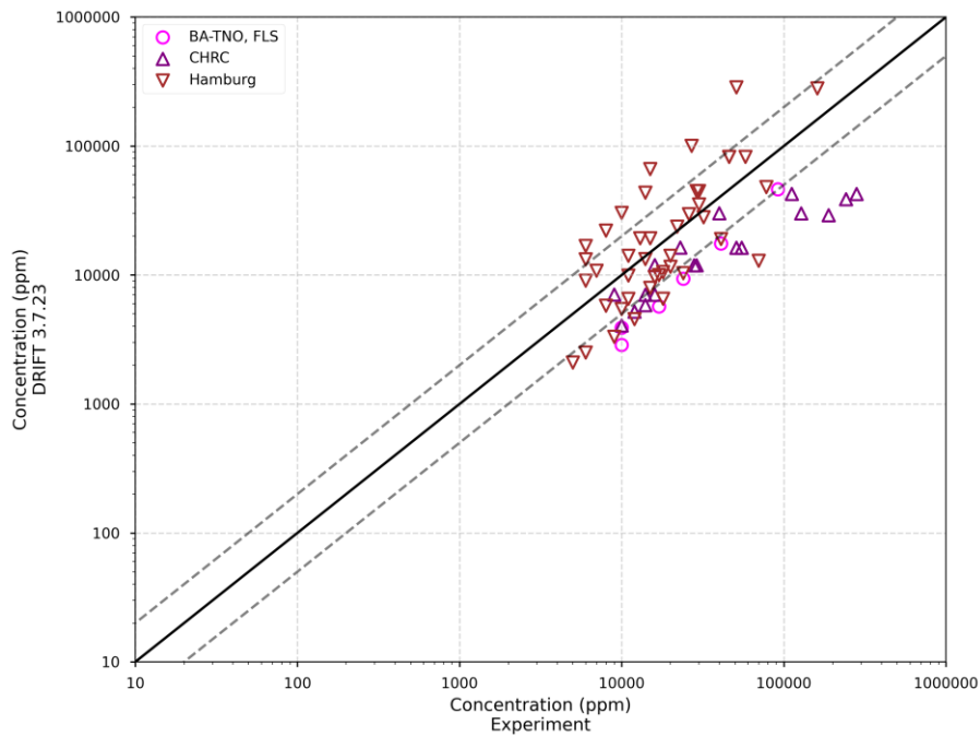
Figure 25 Long-time averaged concentration data scatter for all wind-tunnel trials. Solid line indicates where predicted is equal to measured. Dashed lines indicate a factor of two under- and overprediction.
