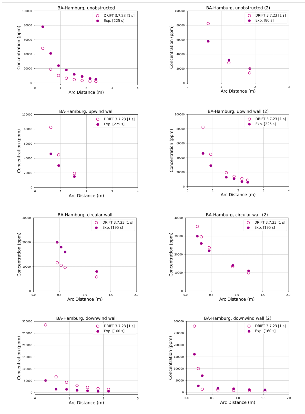
Figure 2 presents a comparison of the DRIFT 3.7.23 concentration predictions with the BA-Hamburg experimental data. In the first BA-Hamburg unobstructed trial, DRIFT underpredicts concentrations by approximately a factor of 2. This may be due to increased dilution over the source from the model, although the predictions for the second unobstructed trial look reasonable.
