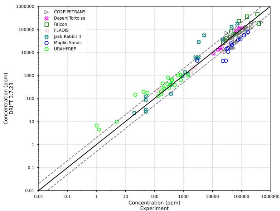
Figure 23 Short-time averaged concentration data scatter for all field trials. Solid line indicates where predicted is equal to measured. Dashed lines indicate a factor of two under- and overprediction.
