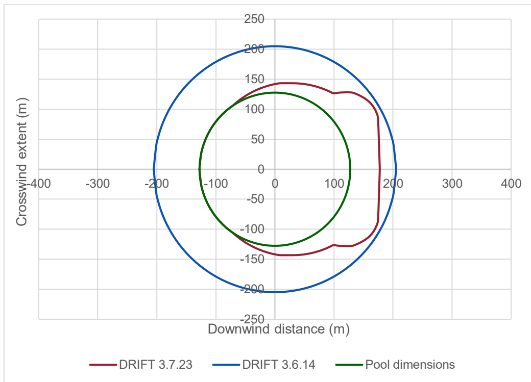
Figure 31 LFL isopleths predicted by DRIFT 3.7.23 and DRIFT 3.6.14 for a major joint failure of the vessel modelled in D4.3 weather conditions with dry soil. The dimensions of the pool source are also shown.
