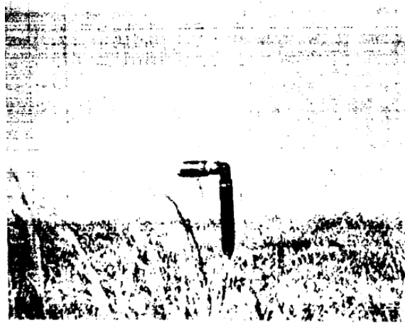
Figure 16 Release configuration for the Prairie Grass experiments – a 50 mm diameter pipe, with the orifice orientated parallel to the floor. Image taken from Barad (1958).
