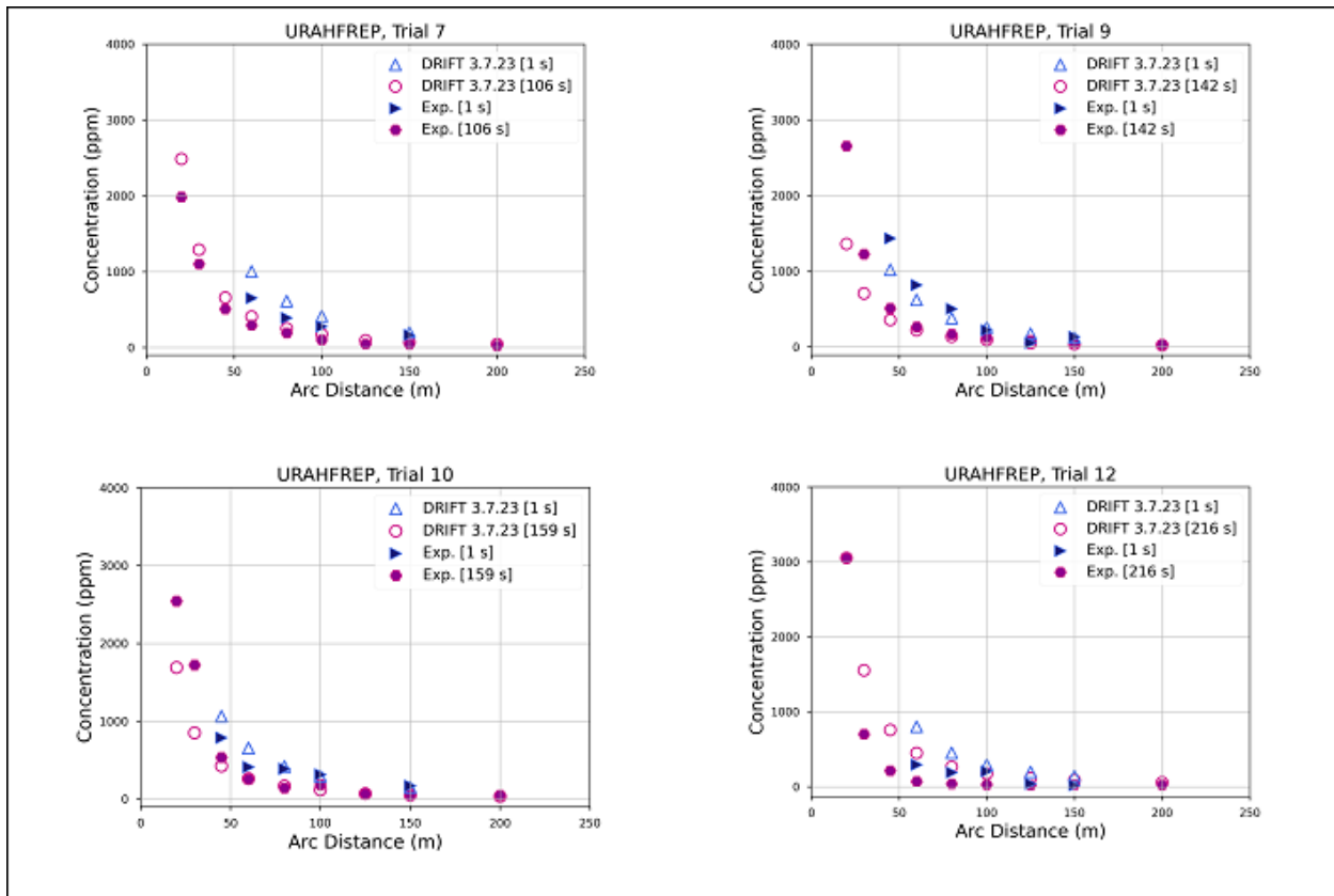
Figure 22 Observed and predicted maximum arcwise concentration data for URAHFREP. Square brackets indicate averaging time.
