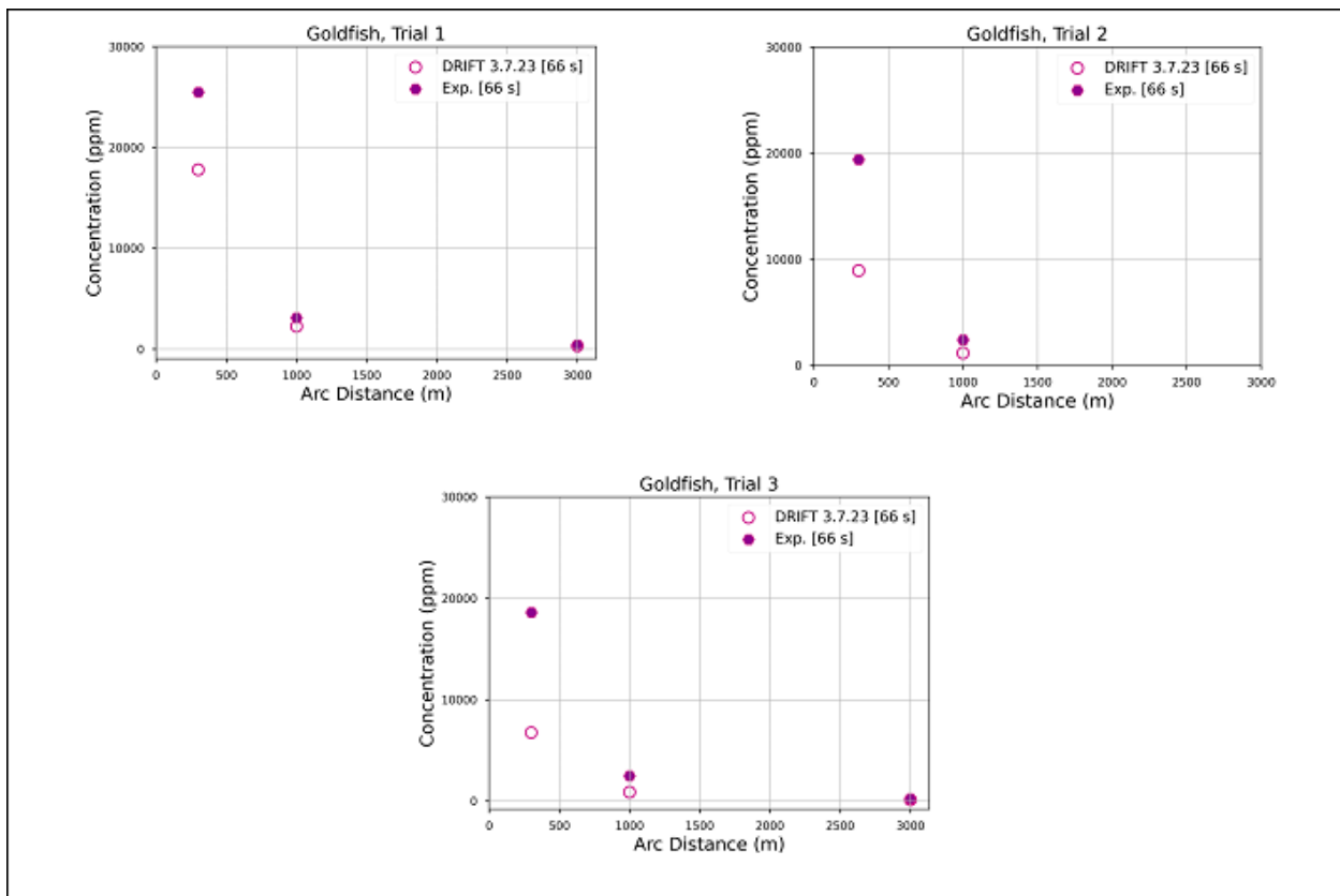
Figure 20 presents the DRIFT 3.7.23 predictions against Goldfish experimental data. For trials 2 and 3, DRIFT underpredicts concentration data at the first sensor by roughly a factor of 2. Better agreement is obtained further downwind, and for trial 1.
