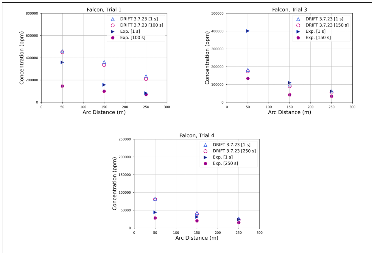
Figure 10 Observed and predicted maximum arcwise concentration data for Falcon. Square brackets indicate averaging time.
