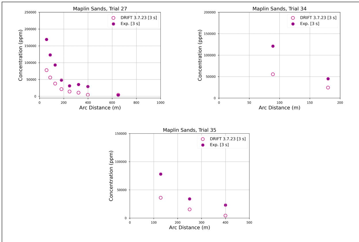
Figure 6 Observed and predicted maximum arcwise concentration data for Maplin Sands. Square brackets indicate averaging time.
