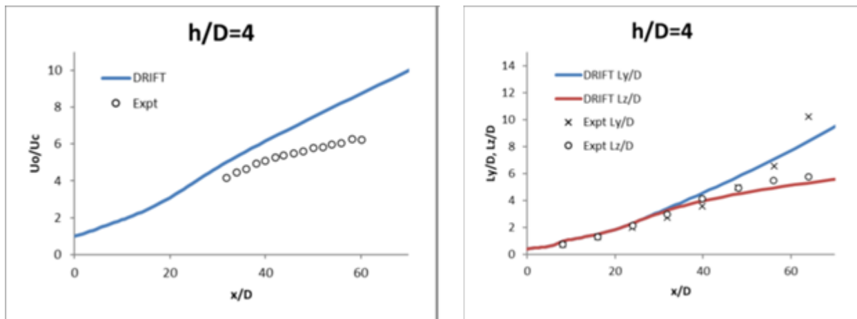
Figure 35 DRIFT 3.7.22 predictions of velocity and plume dimensions for h/D = 4 compared with Davis and Winarto (1980) data. Reproduced from Figure 2-9 of Tickle (2025c).
