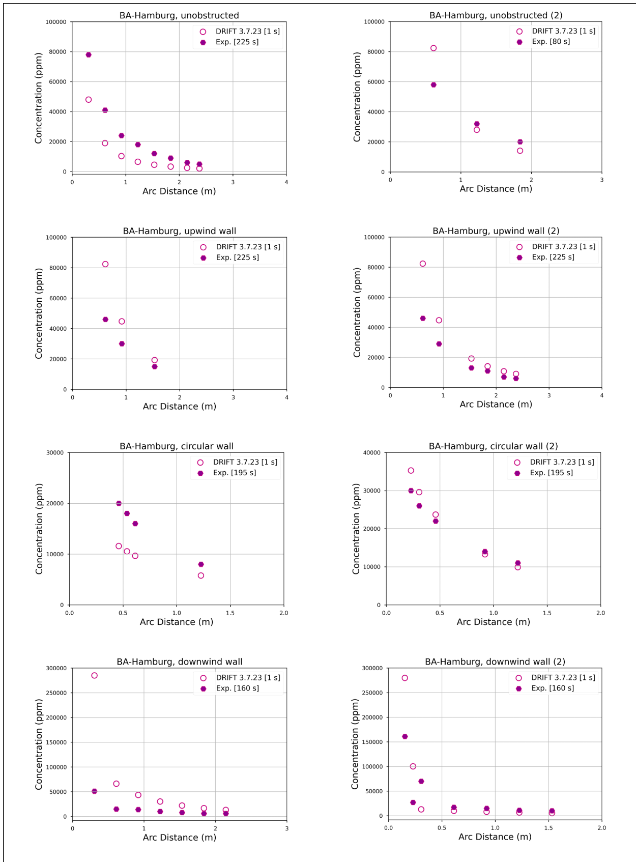
Figure 2 Observed and predicted maximum arcwise concentration data for BA-Hamburg wind-tunnel trials. Square brackets indicate averaging time.
