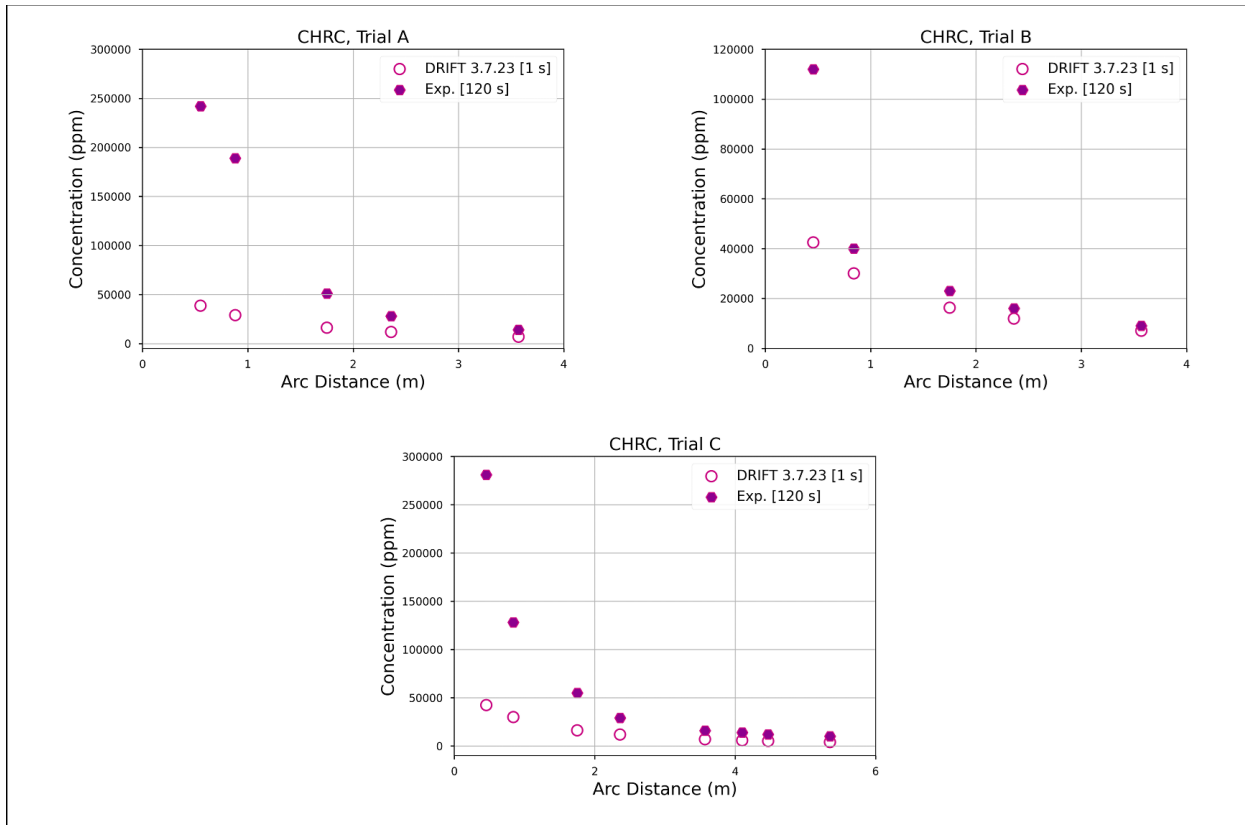
Figure 5 Observed and predicted maximum arcwise concentration data for CHRC. Square brackets indicate averaging time.
