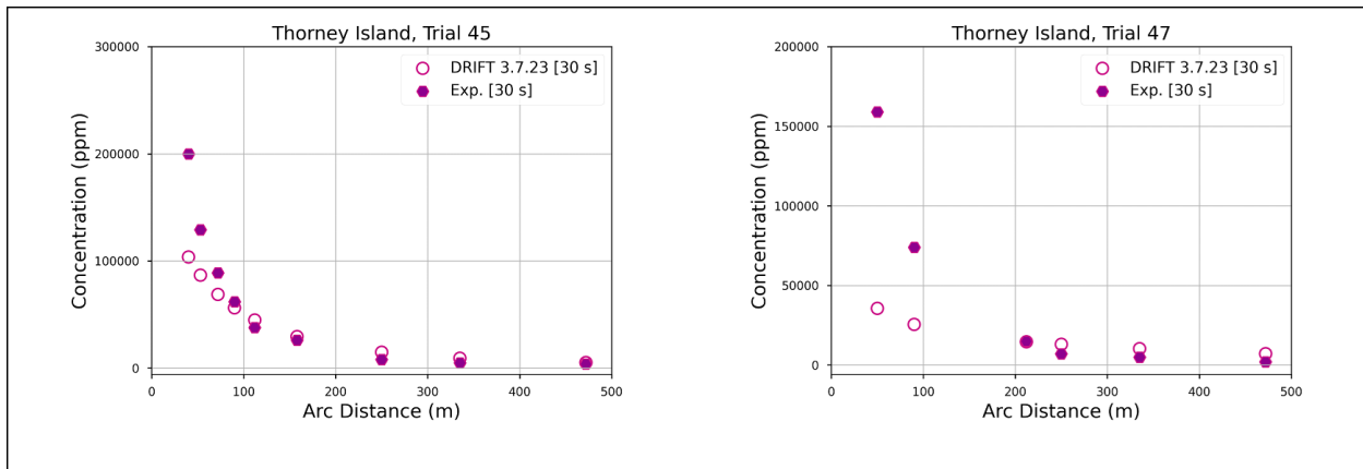
Figure 12 Observed and predicted maximum arcwise concentration data for Thorney Island. Square brackets indicate averaging time.
