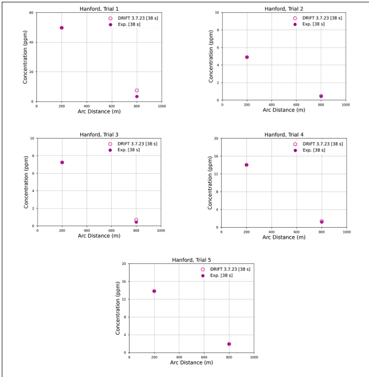
Figure 15 presents DRIFT 3.7.23 predictions for Hanford trials 1, 2, 3, 4 and 5. Given the scaling at the first downwind position of 200 m, only the 800 m arc data can be used to judge the performance of DRIFT. It can be seen that DRIFT predictions are in close agreement with experiment for the arc at 800 m, apart from a slight overprediction of roughly a factor of 2 for trial 1.
