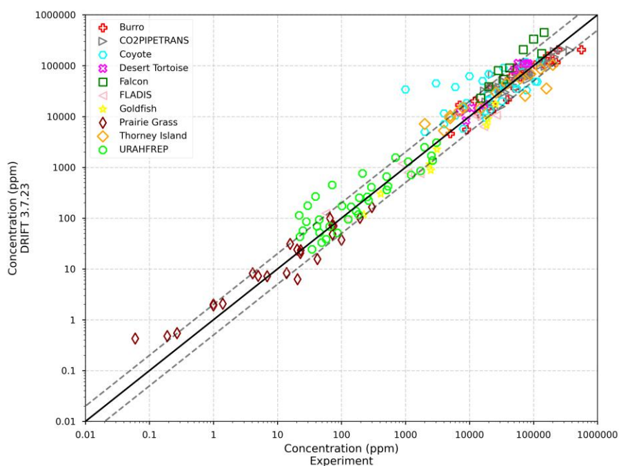
Figure 24 Long-time averaged concentration data scatter for all field trials. Solid line indicates where predicted is equal to measured. Dashed lines indicate a factor of two under- and overprediction.
