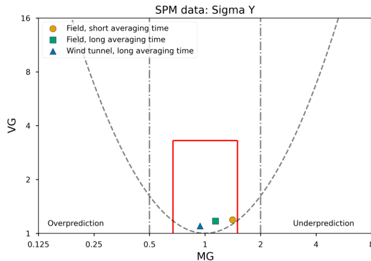
Figure 30 Geometric variance (VG) versus geometric mean bias (MG) based on cloud width data.
