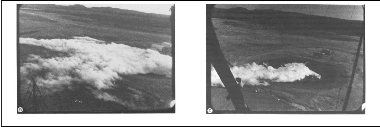
Figure 7 Left: snapshot of the vapour cloud in Burro 8 at 160 s demonstrating bifurcation. Right: Burro 6 after a quasi-steady state has been achieved. Both images from Ermak et al. (1982).
