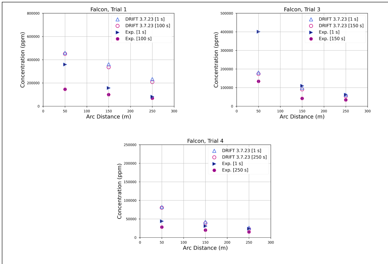
Figure 10 presents a comparison of the DRIFT 3.7.23 predictions with the Falcon experimental data. There is slight overprediction of concentration in trial 1, but otherwise the DRIFT 3.7.23 predictions are in close agreement with the experimental data.
