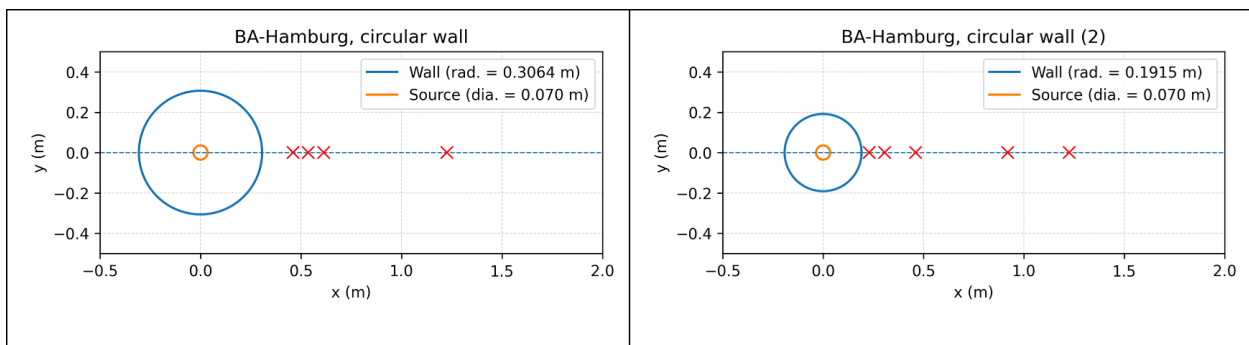
Figure 3 Scale drawings of the two circular wall geometries from the BA-Hamburg trials. Sensor locations are marked with a red cross.
