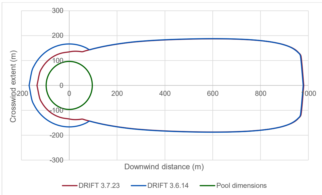
Figure 32 LFL isopleths predicted by DRIFT 3.7.23 and DRIFT 3.6.14 for a major joint failure of the vessel modelled in D4.3 weather conditions with wet soil. The dimensions of the pool source are also shown.
