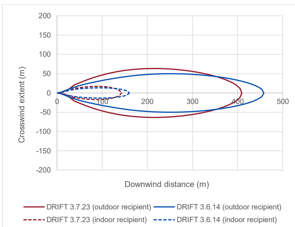
Figure 33 SLOT DTL isopleths obtained for indoor and outdoor recipients for a chlorine release from a 50 mm hole in liquid pipework in F2.4 weather conditions, assuming a release duration of 1 minute. Dispersion of the initial airborne component is shown.
