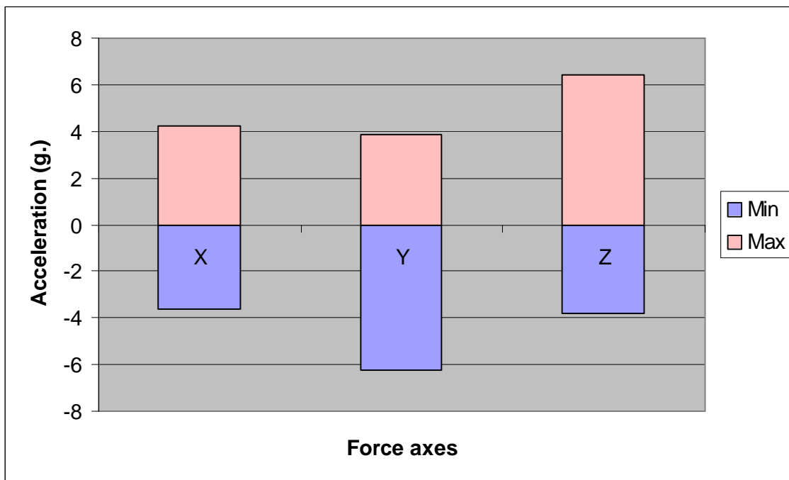
Figure 2. Peak measured forces from the database entries.
