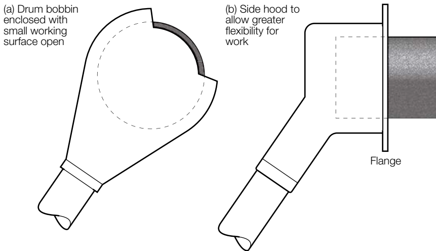
Figure 1 LEV hoods for drum/bobbin sanders
