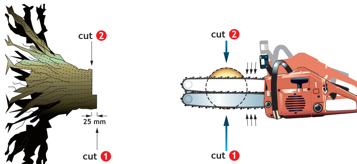
Figure 1 Severing cuts
