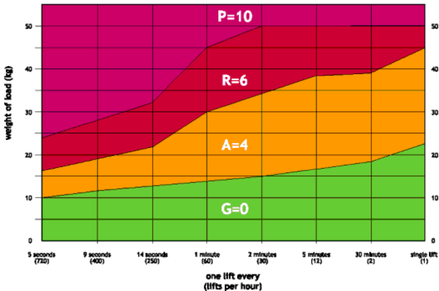
Load/frequency graph for Lifting Operations
