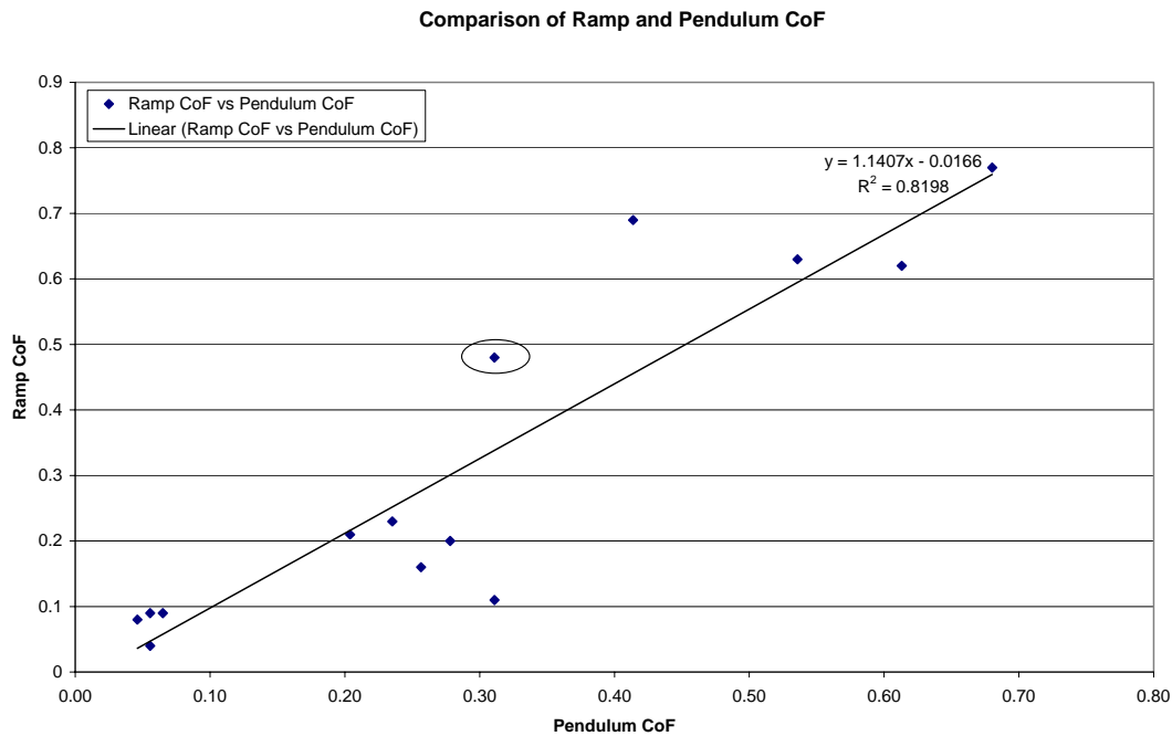
Figure 3.2 Graph comparing the coefficient of friction results obtained in water wet conditions using the ramp and pendulum test methods.
