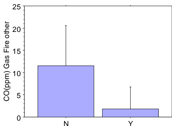
Figure 14 : Mean carbon monoxide concentrations measured from gas fire (other) split by maintenance in the last year or not.
