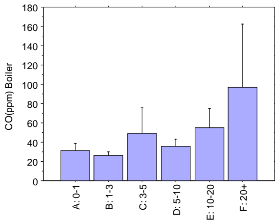
Figure 6 : Mean carbon monoxide concentration measured from boilers split by their age range.
