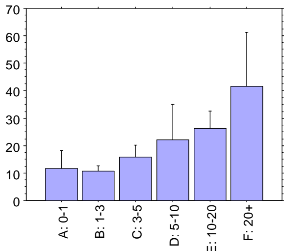
Figure 3 : Mean carbon monoxide concentration measured from cookers split by their age range.
