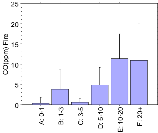
Figure 10 : Mean carbon monoxide concentrations measured from Gas Fires (main room) split by their age range.
