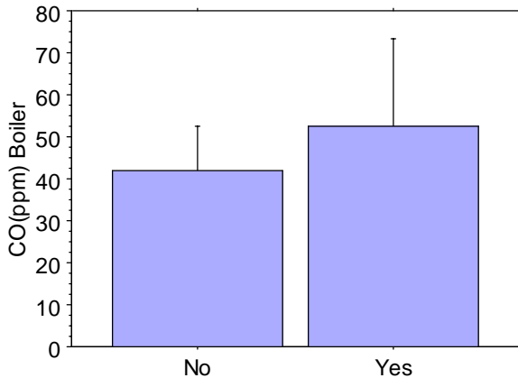
Figure 7 : Mean carbon monoxide concentration measured from boilers split by if the owners had a maintenance certificate or not.
