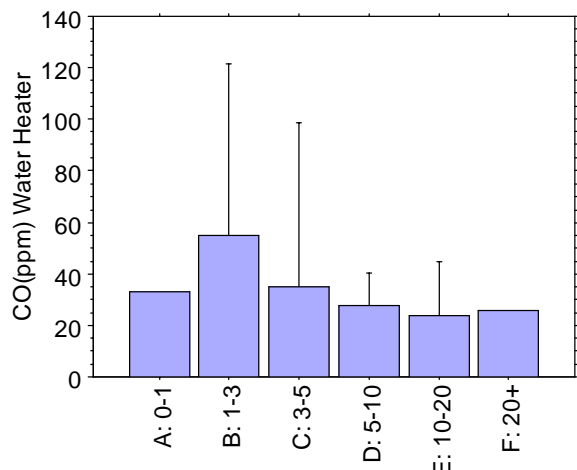
Figure 16 : Mean carbon monoxide concentrations measured from Water Heaters split by their age range.
