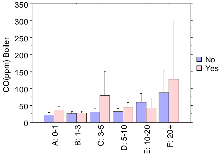
Figure 8 : Mean carbon monoxide concentration measured from boilers split by age and if the owners had a maintenance certificate or not.
